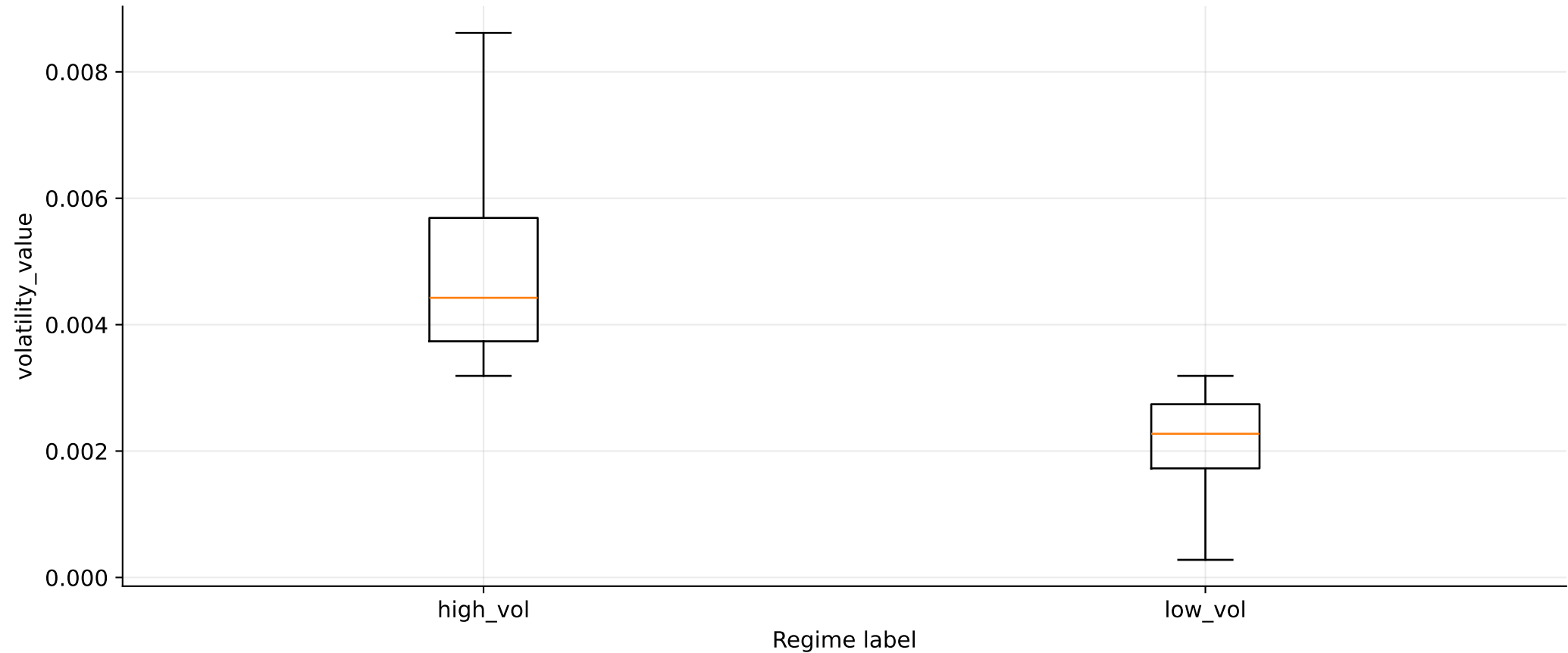
Volatility distribution by regime - ETHUSDT 15m quantile
